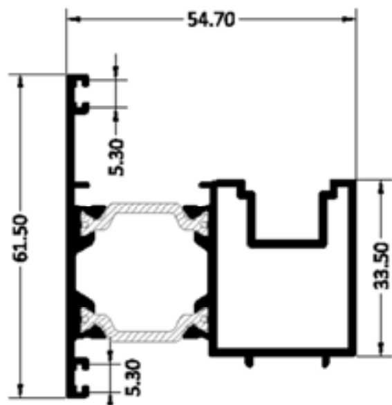
INVERSOR RECTO CAN/16
