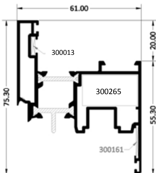
HOJA VENTANA RECTA CAN/16
