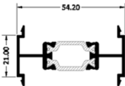
UNION DE MARCOS 54 MM CAN/16
