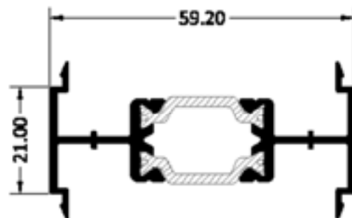
UNION DE MARCOS 59 MM CAN/16
