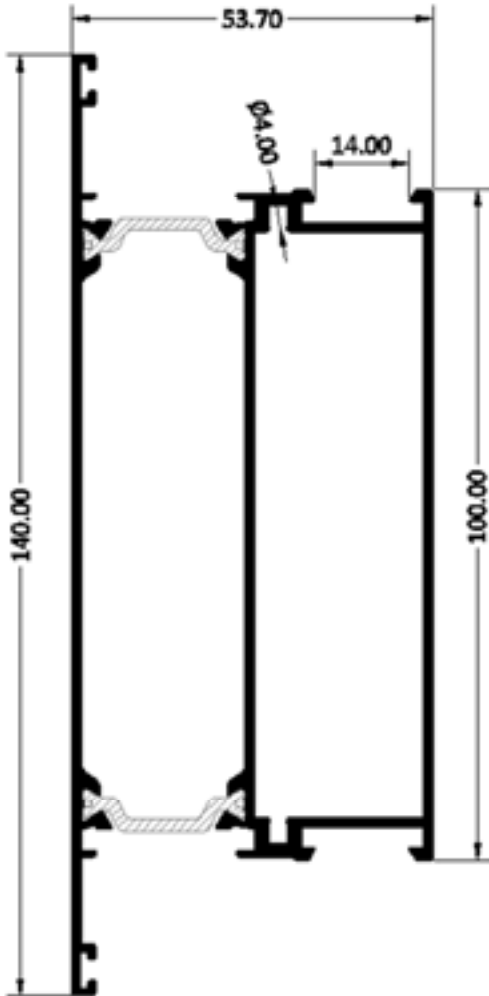
PARTELUCES 140 MM CAN/16
